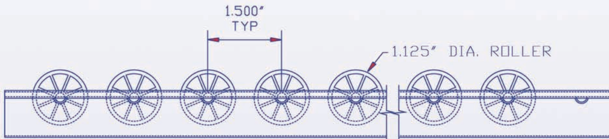
SIDE VIEW OF CARTON FLOW TRACK
