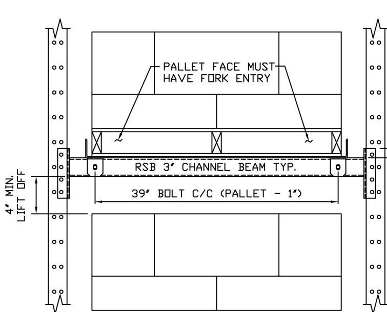
SECTION @ RAIL SUPPORT BEAM
