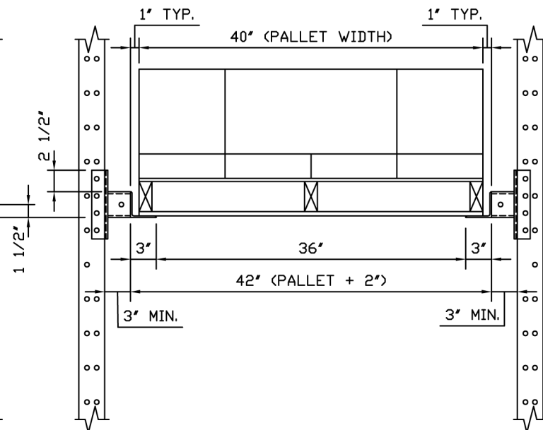
SECTION @ DA37 DRIVE IN ARM
