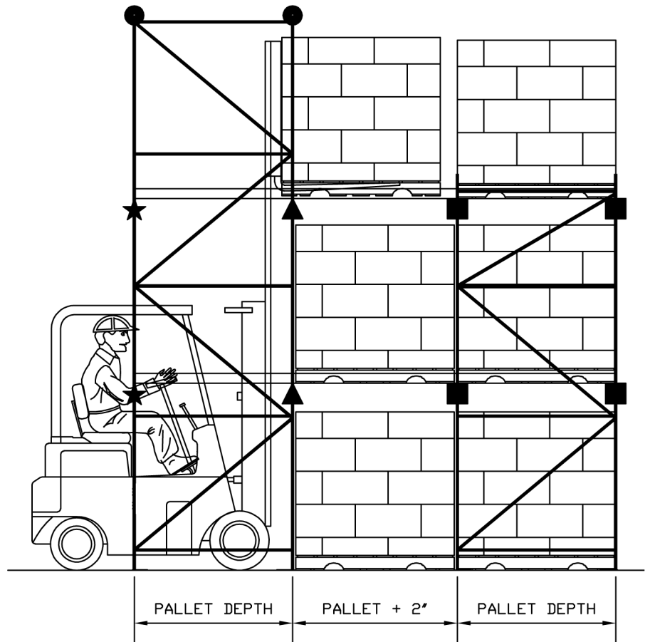
STANDARD THREE DEEP DRIVE IN
