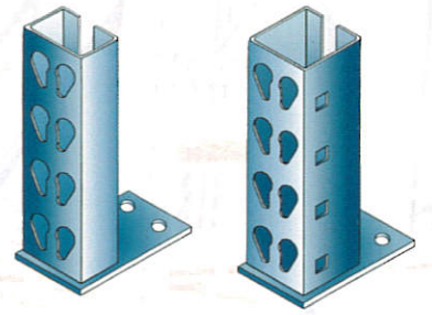
3 x 1 5/8" 3 x 3" INTERCHANGEABLE OPEN COLUMN
