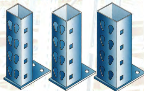
3 x 2" 3 x 3" 4 x 3" INTERCHANGEABLE CLOSED TUBE
