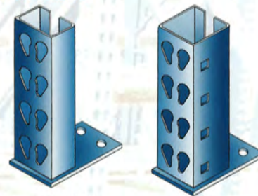
3 x 1 5/8" 3 x 3" INTERCHANGEABLE OPEN COLUMN
